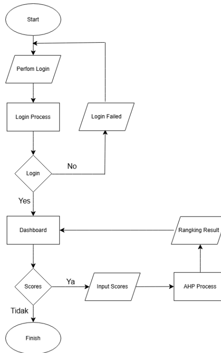
Fig. 2. Flowchart System
