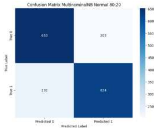
Gambar 10. Confusion Matrix Multinomial NB
