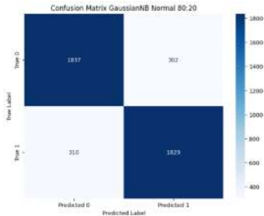
Gambar 9. Confusion Matrix Gaussian Nb
