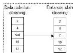
Gambar 2. Clean Data
