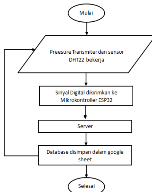
Gambar 2. Flowchart
