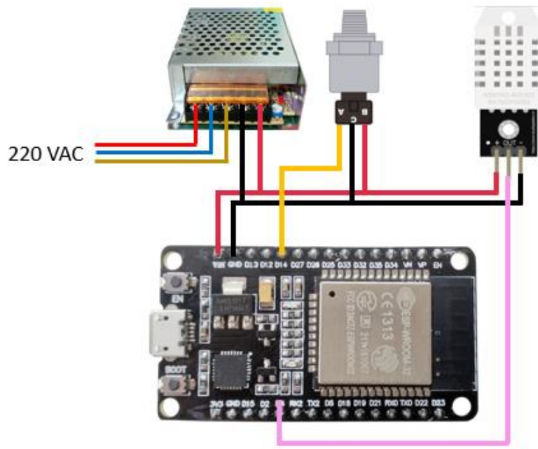
Gambar 3. Wiring Diagram
