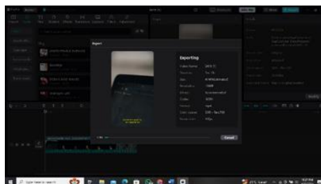
Gambar 6. Rendering
