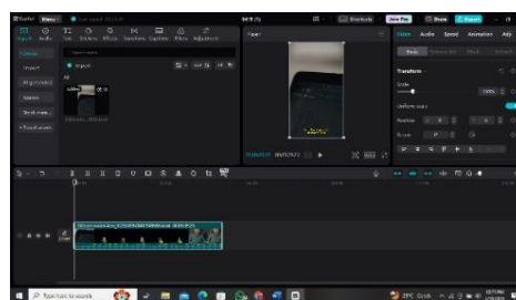
Gambar 4. Editing Video
