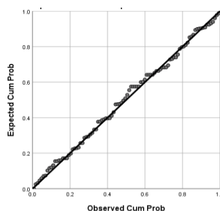
Gambar 1. Normal Probability Plot
