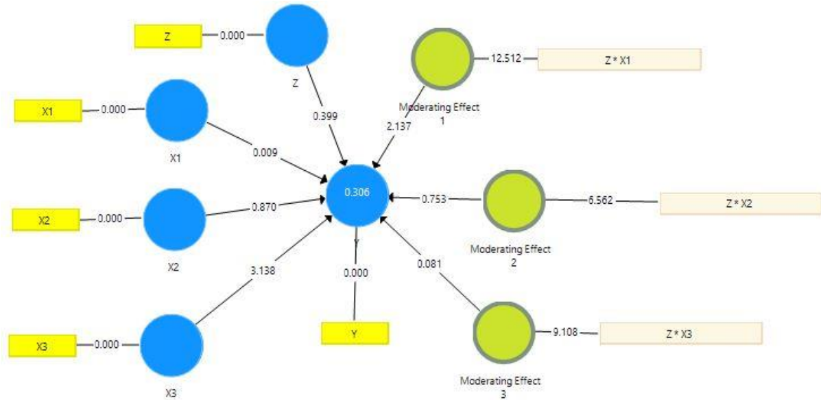
Gambar 1. Hasil bootstrapping
