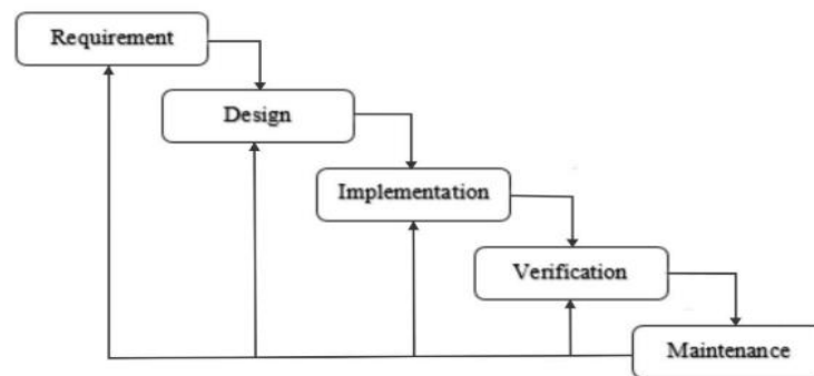
Gambar 1. Metode Waterfall.
