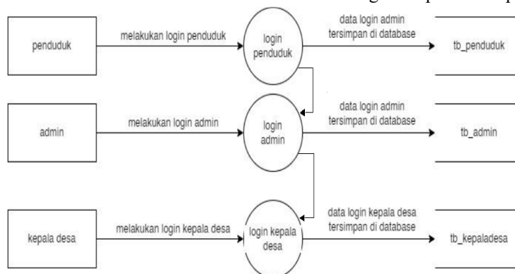
Gambar 4. Data Flow Diagram Level 2 Proses Login.
