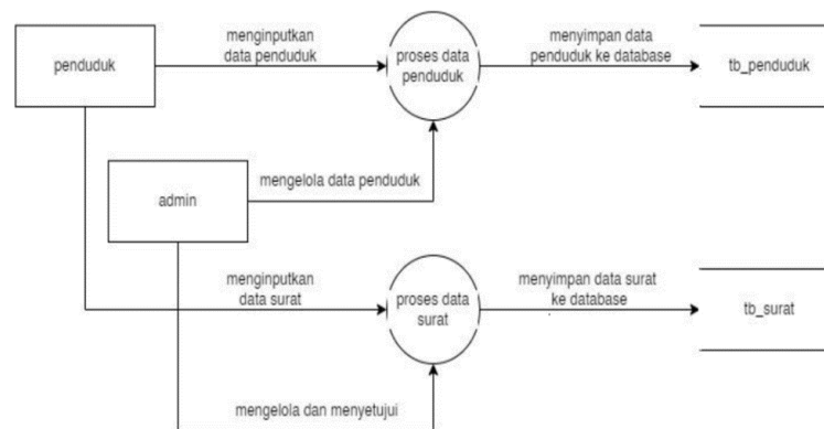
Gambar 5. Data Flow Diagram Level 2 Proses Input Data.
