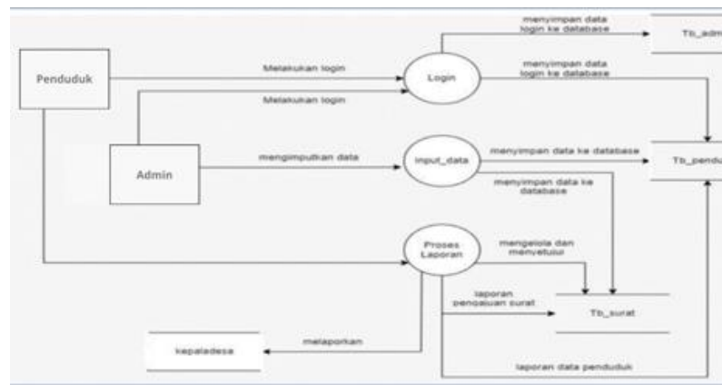
Gambar 3. Data Flow Diagram Level 1.
