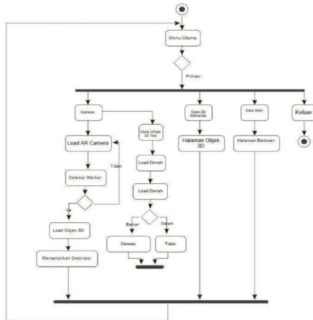
Gambar 5. Activity Diagram
