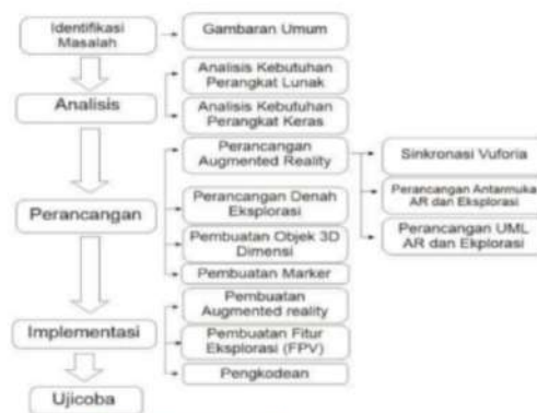
Gambar 1. Metode Waterfall
