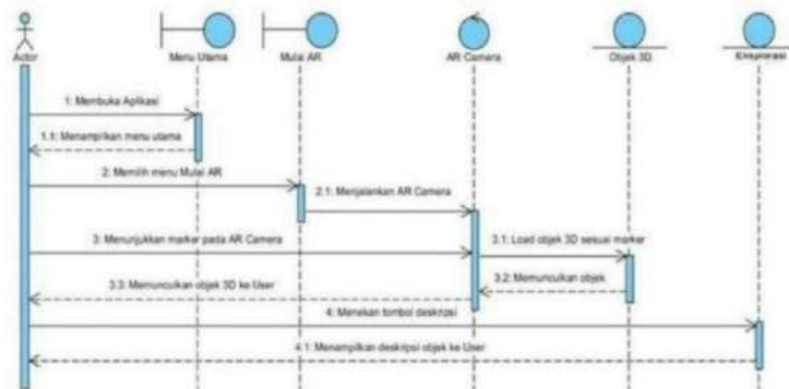
Gambar 6. Sequence Diagram
