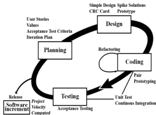
Gambar 1. Diagram Proses Metode Extreme Programming
