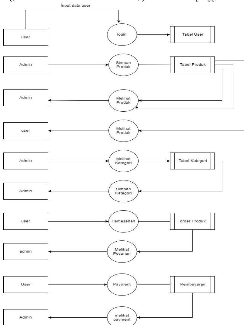
gambar 3, Dfd Level 1
