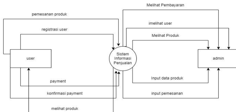
gambar 2, Dfd Level 0
