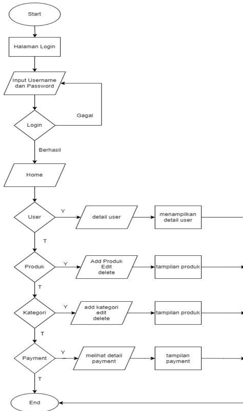
Gambar 1, Flowchart Admin
