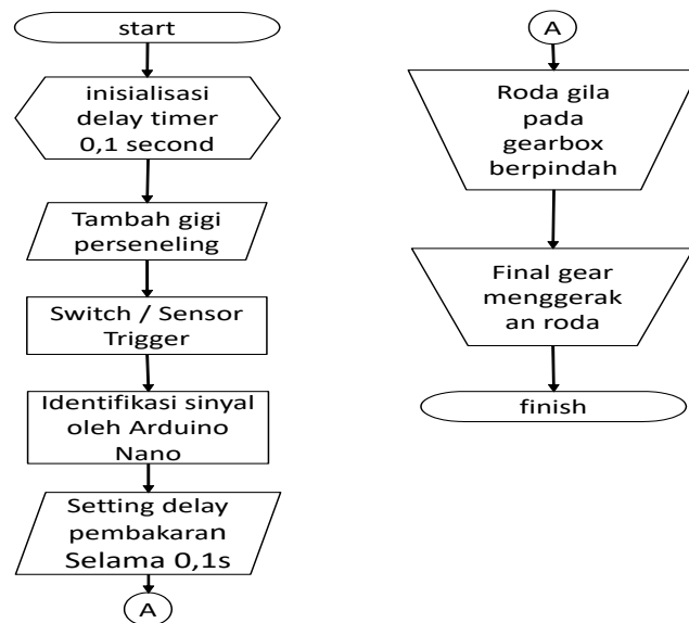
Gambar 8. Flowchart [8]
