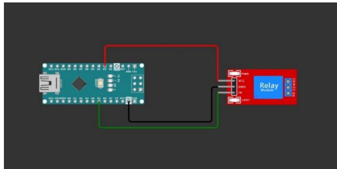
Gambar 6. Rangkaian Relay [6]
