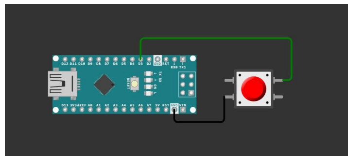
Gambar 5. Rangkaian Trigger [5]
