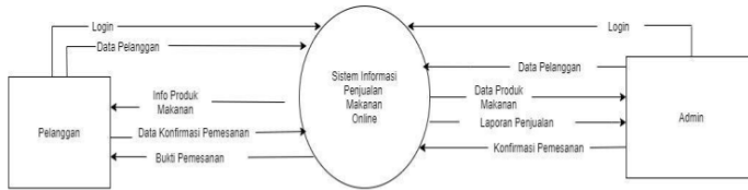
Gambar 3. DFD Level 0
