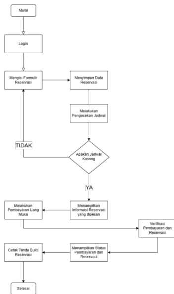
Gambar 2. Flowchart User
