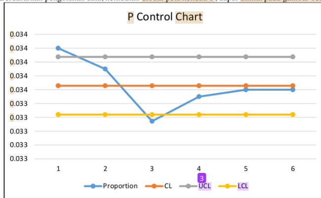
Gambar 4 Peta Kendali P Chart
