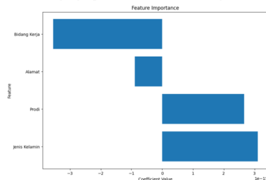
Gambar. 4. Hasil Visualisasi Feature Importance.
