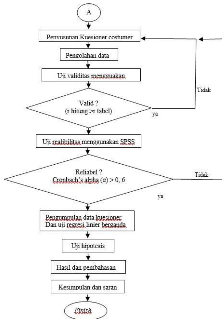
Gambar 1 Flowchart Diagram
