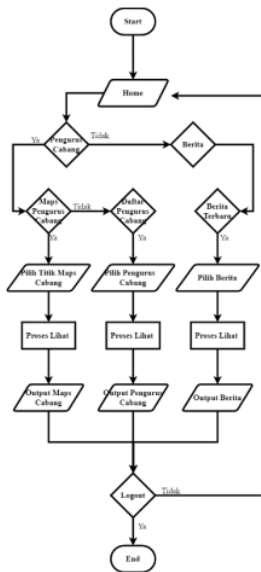
10 Gambar 3.3 Flowchart User
