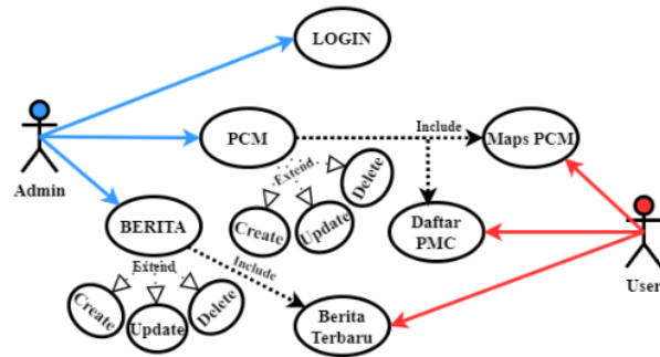
Gambar 3.4 Uce Case Diagram
