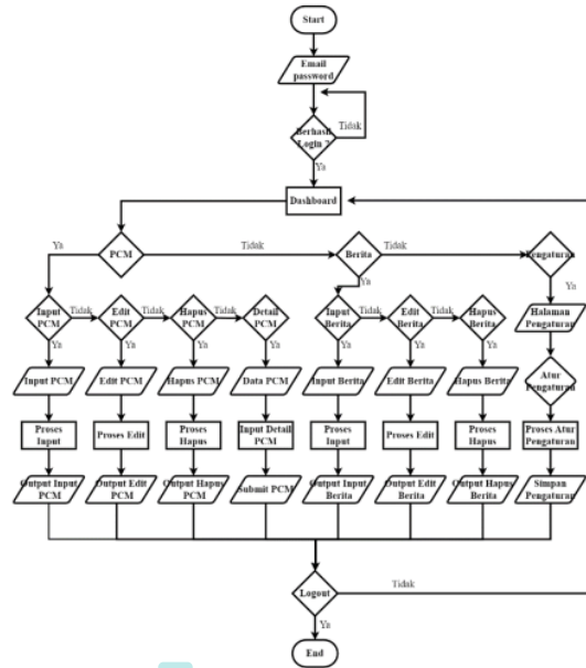
16 Gambar 3. 2 Flowchart Admin
