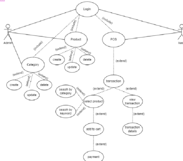
Gambar 3.3 Uce Case Diagram
