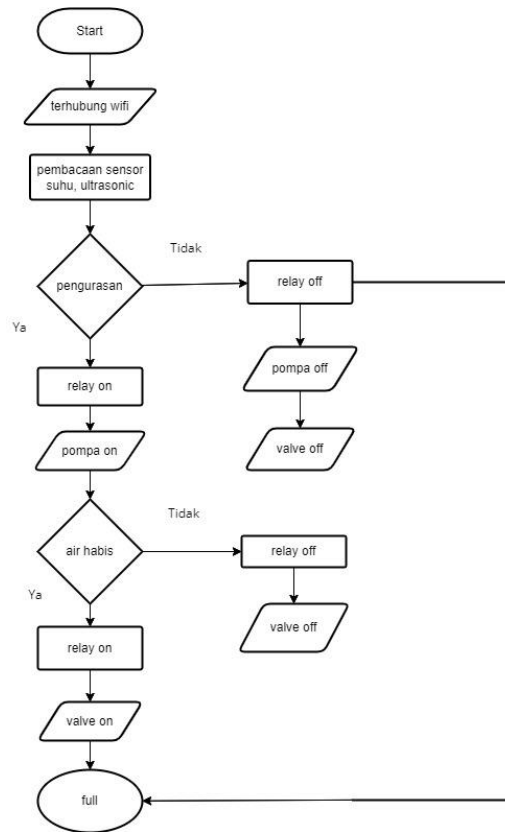
Gambar 4. Diagram Alur Sistem
