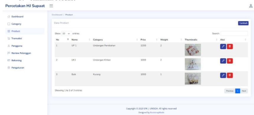
Gambar 3.7 Halaman Product
