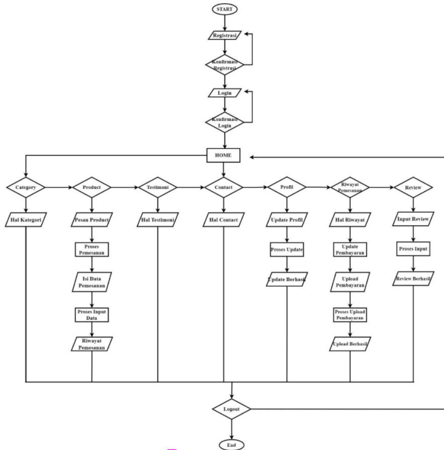
2 Gambar 3.2 Flowchart User
