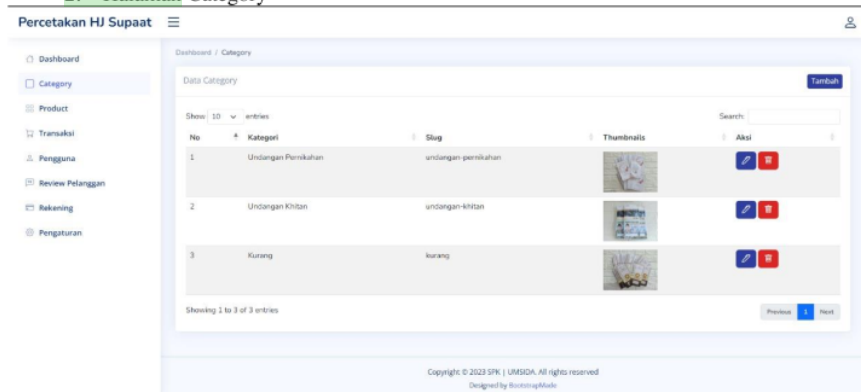
Gambar 3.6 Halaman Category
