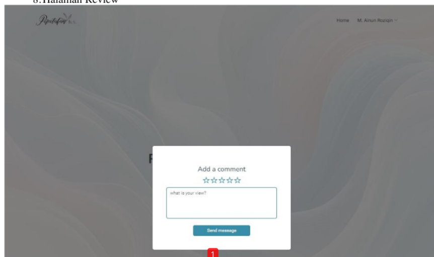
Gambar 3.20 Halaman Review
