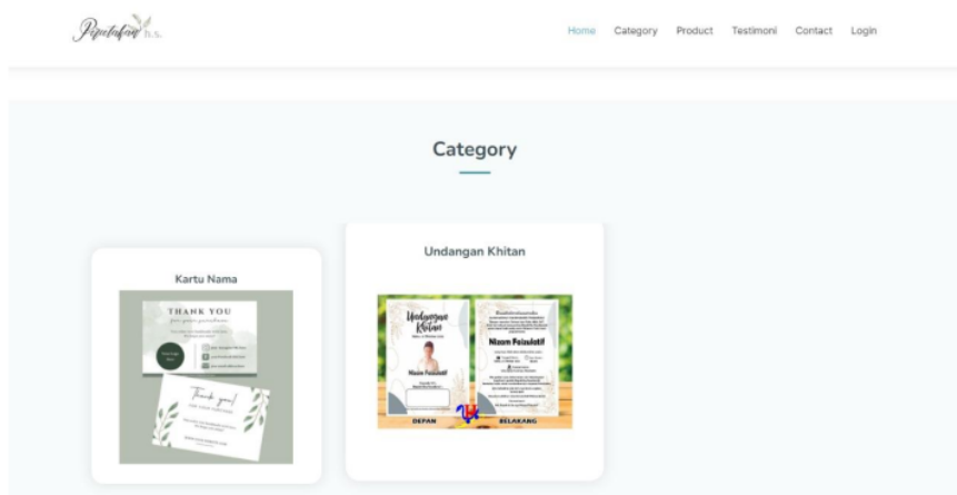
Gambar 3.14 Halaman Category
