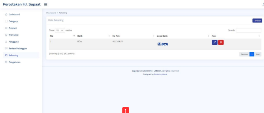
Gambar 3.11 Halaman Rekening
