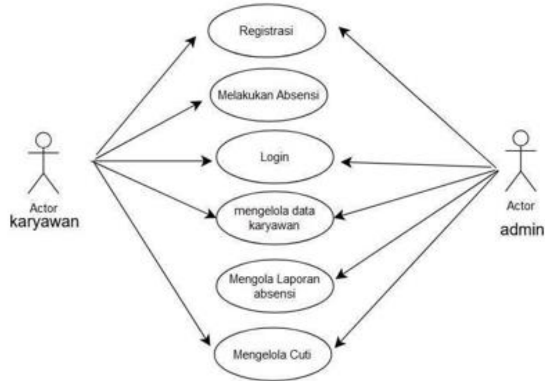
Gambar 3.3 Usecase Diagram
