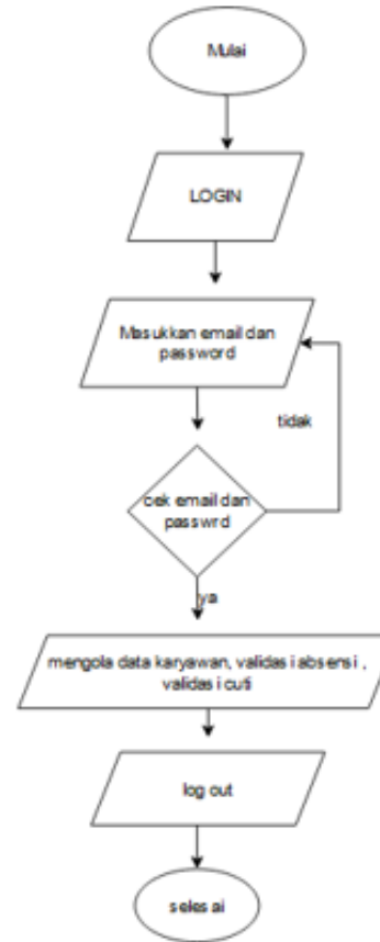
Gambar 3.1 Flowchart Admin
