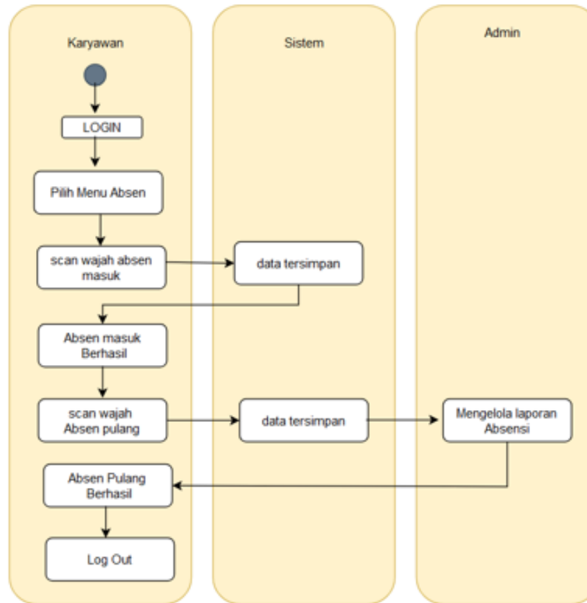
Gambar.3.4 Activity Diagram
