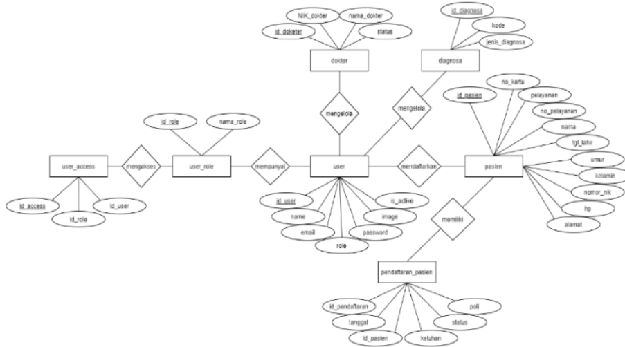
Gambar Error! No text of specified style in document..5 Entity Relation Diagram
