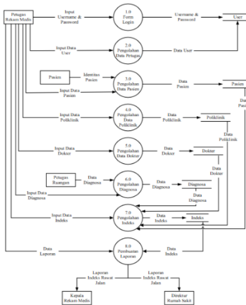
Gambar Error! No text of specified style in document..A Data Flow Diagram
