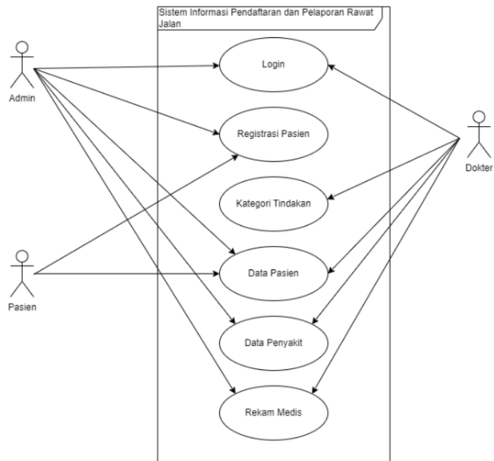
17 Gambar Error! No text of specified style in document..2 Use Case Diagram
