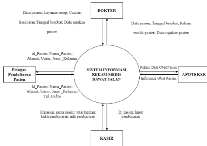
Gambar Error! No text of specified style in document..3 Diagram Konteks
