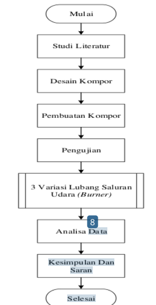
Gambar 2.1. Flowchart Penelitian
