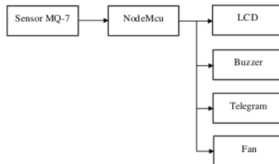
Gambar 1. Blok Diagram
