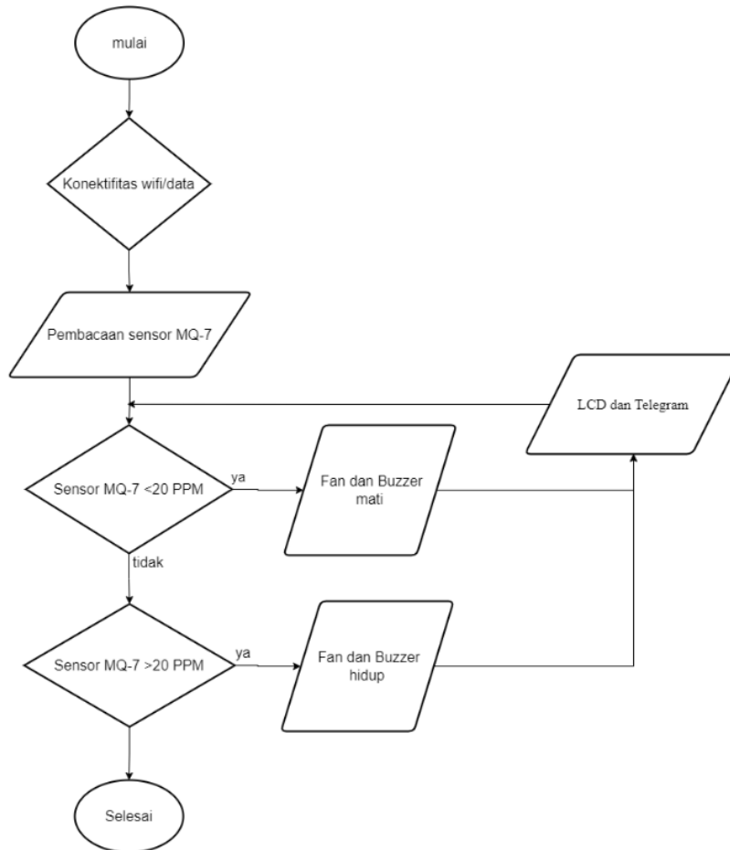
Gambar 2. Flowchart
