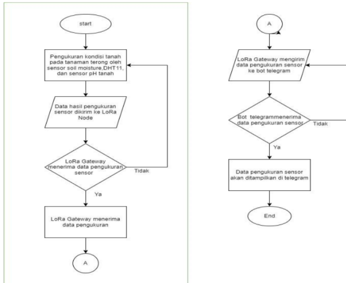
Gambar 3. Flowchart Implementasi Sistem
