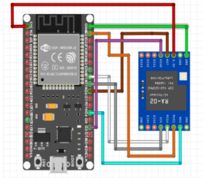
Gambar 2. Rangkaian Receiver
