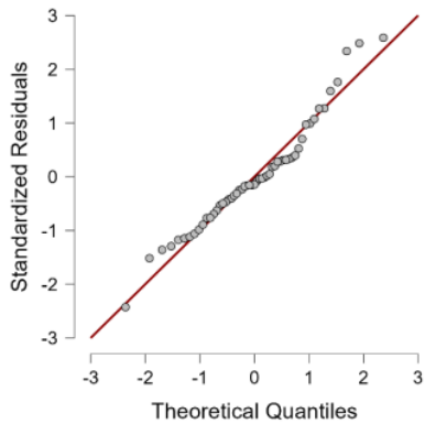
Gambar 1. Q-Q Plot Standardized Residuals
