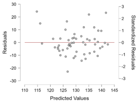
Gambar 2. Residuals vs. Predicted
