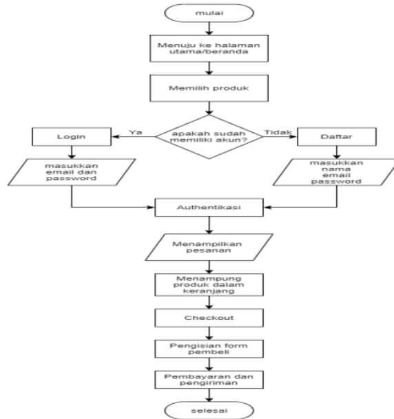
19 Gambar 2.2. Flowchart
