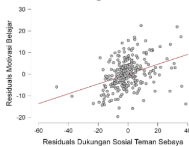
Partial Regression Plots
