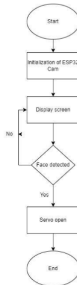
Gambar 3. Flowchart
