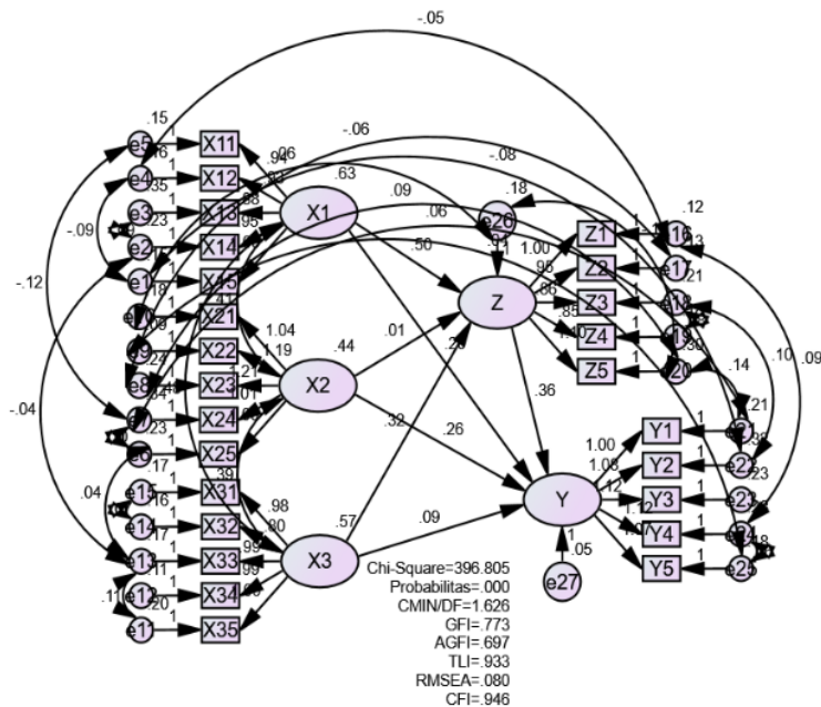
Gambar 4.2 Hasil Analisis SEM (Saturated Model)
