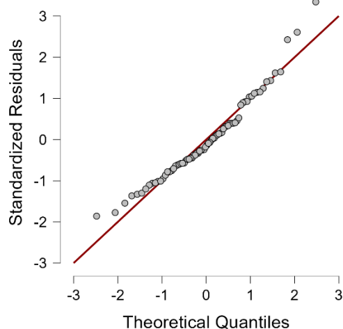
Gambar 2. Q-Q Plot Standardized Residuals
