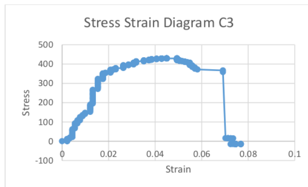
Gambar 19. Diagram Stress Strain Spesimen C3
