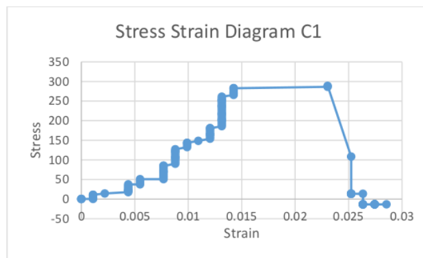
Gambar 17. Diagram Stress Strain Spesimen C1
