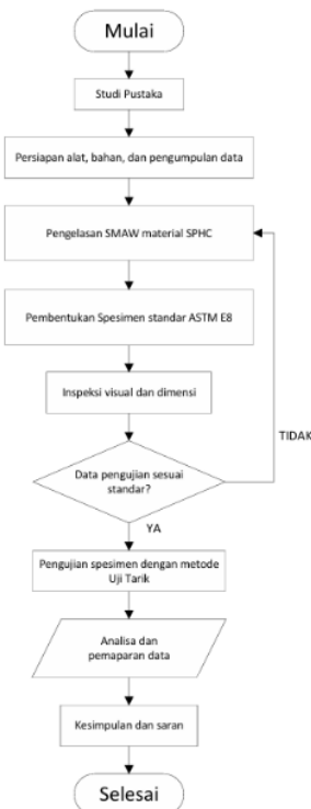
Gambar 6. Diagram Alir Penelitian
