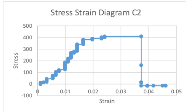
Gambar 18. Diagram Stress Strain Spesimen C2
