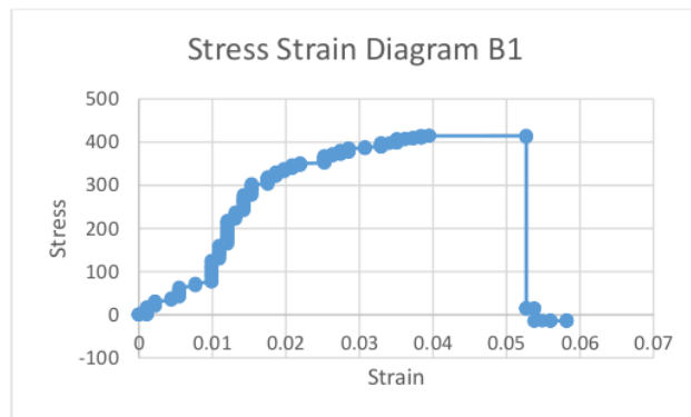
Gambar 14. Diagram Stress Strain Spesimen B1
