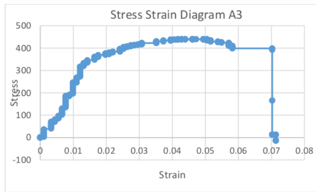
Gambar 13. Diagram Stress Strain Spesimen A3
