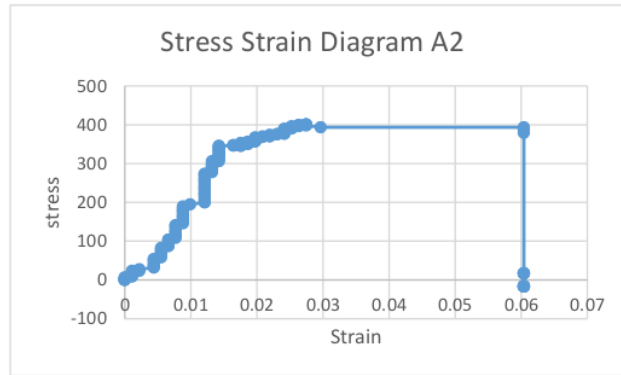
Gambar 12. Diagram Stress Strain Spesimen A2
