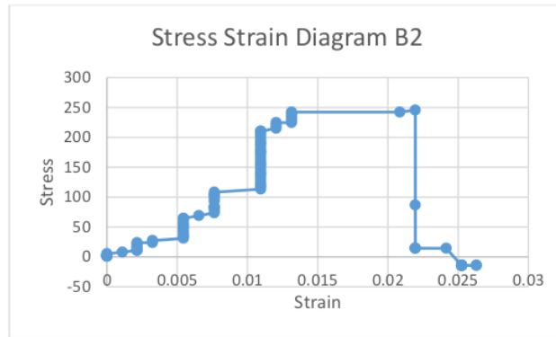
Gambar 15. Diagram Stress Strain spesimen B2
