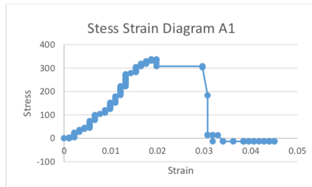
Gambar 11. Diagram Stress Strain Spesimen A1
