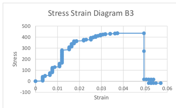
Gambar 16. Diagram Stress Strain Spesimen B3
