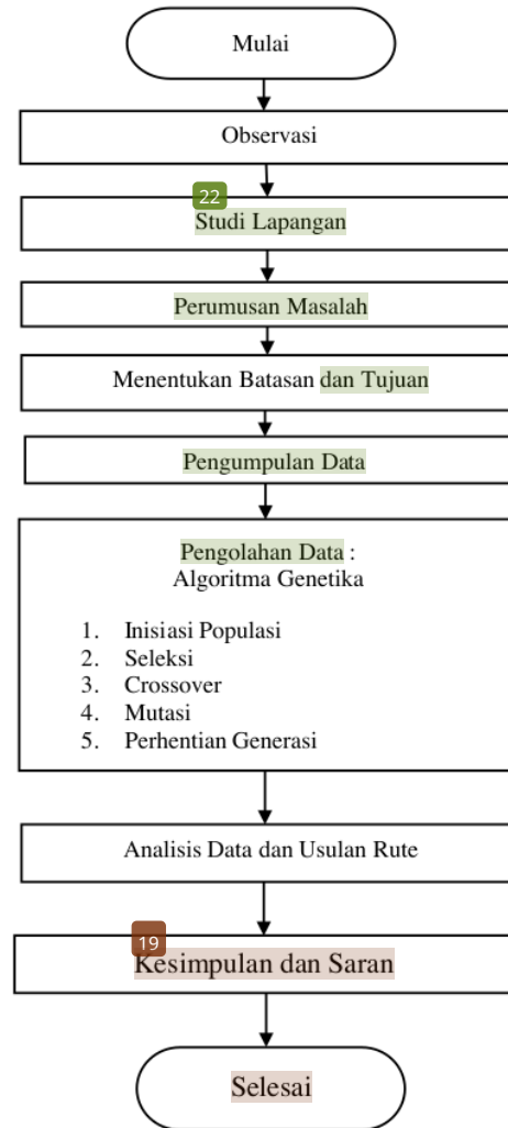
Gambar 1. Flowchart Penelitian
