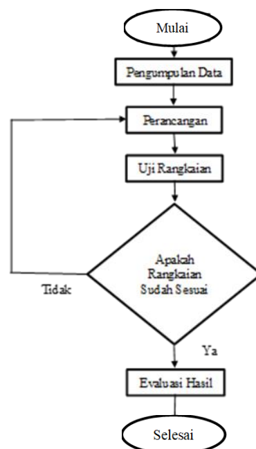
Gambar 1. Flowchart Penelitian
