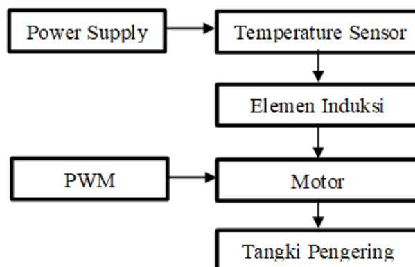
Gambar 3. Diagram Blok
