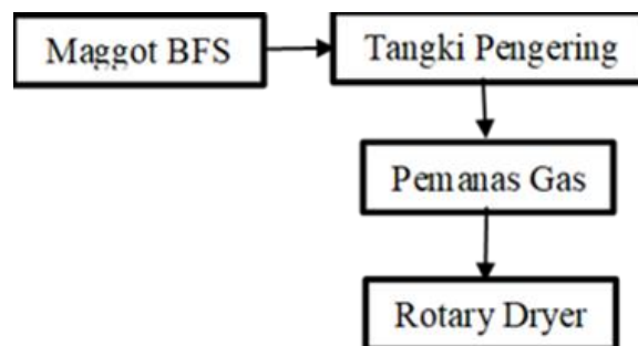
Gambar 2. Blok Diagram Penelitian terdahulu
