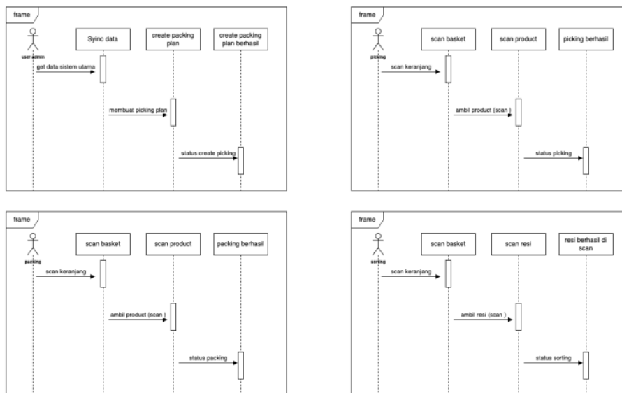
Gambar 7 Sequence Diagram Admin, picker, packer, sortir
