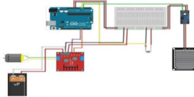
Gambar 1. Wiring Diagram
