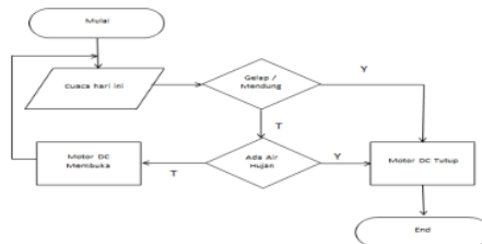
Gambar 3. Diagram Alir
