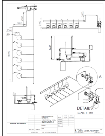
Gambar 1. Drawing Jalur Perpipaan Distribusi Air Mixer
