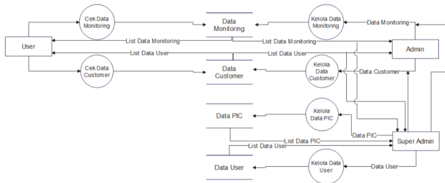
Gambar 3.4 DFD (Data Flow Diagram)
