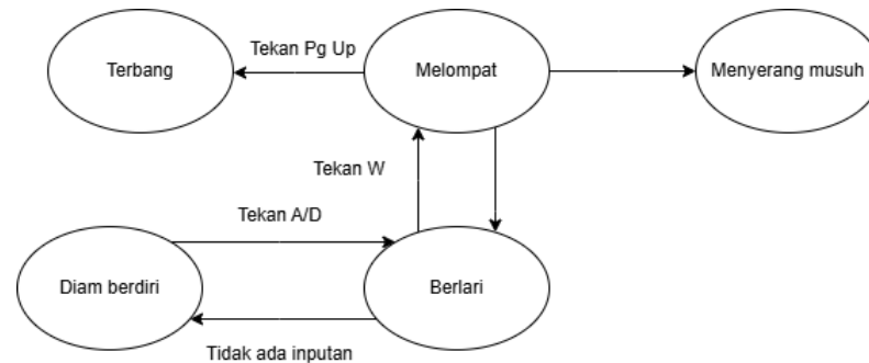
Gambar 4 FSM Player
