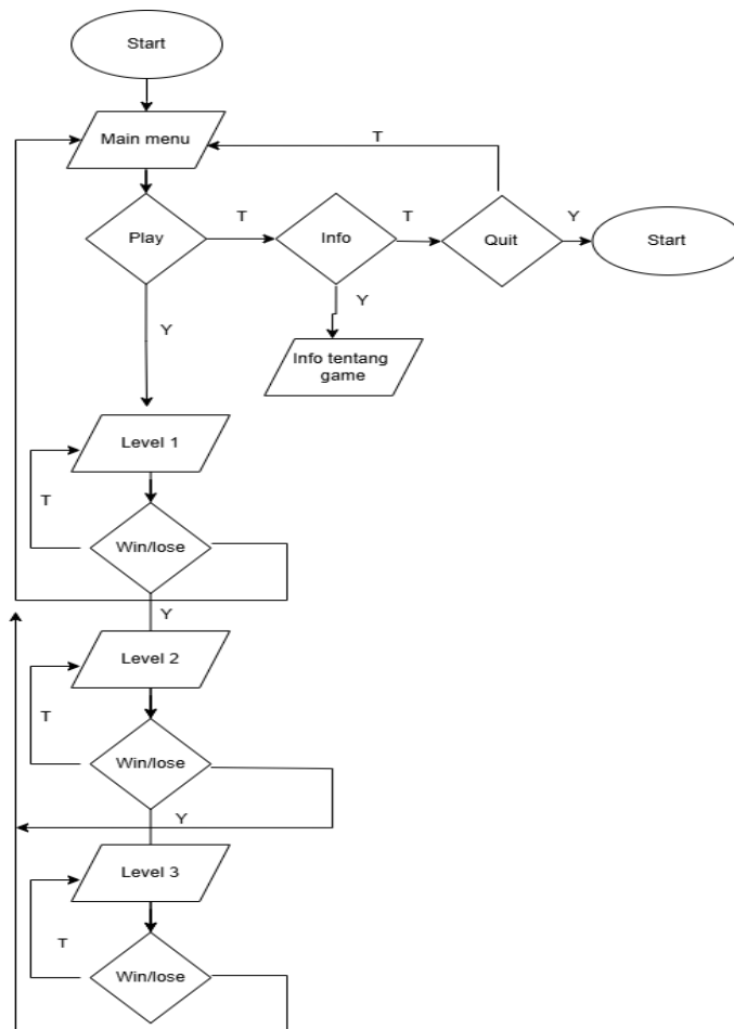
Gambar 2 Flowchart Game
