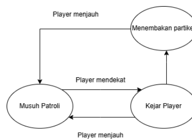
Gambar 3 FSM Boss Monster
