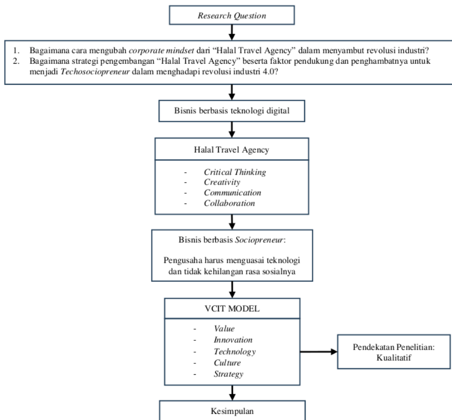
Gambar 2. Research Framework
