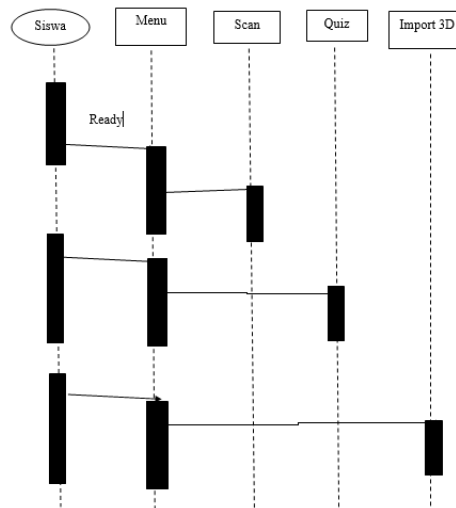
Gambar 4. Sequence Diagram
