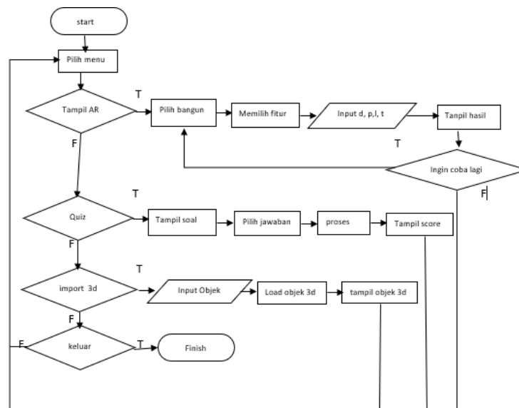
Gambar 2. Flowchart
