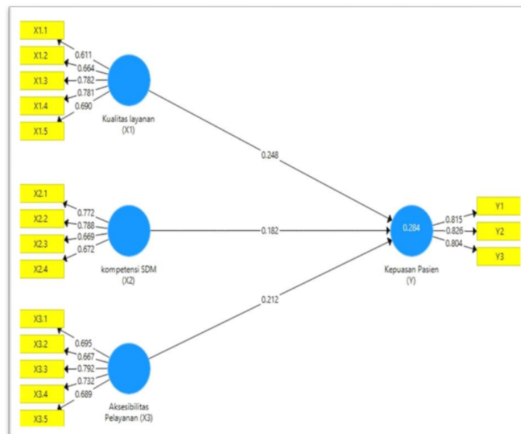
Gambar 1. Model Struktural PLS Algorithm
