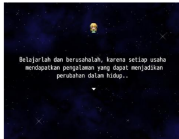
Gambar 7. Ending Game
