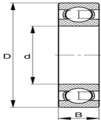
Gambar 4. Sketsa Bearing 6311
