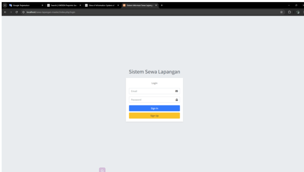
Gambar 3.2 Halaman Login/Register
