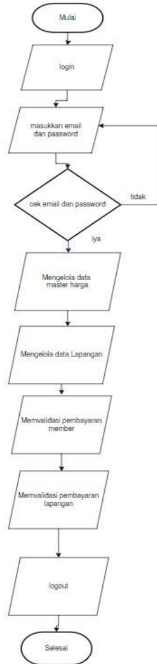
Gambar 2.3 Flowchart Admin
