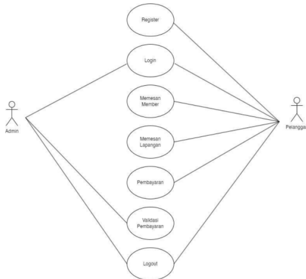
Gambar 2.1 Usecase Diagram
