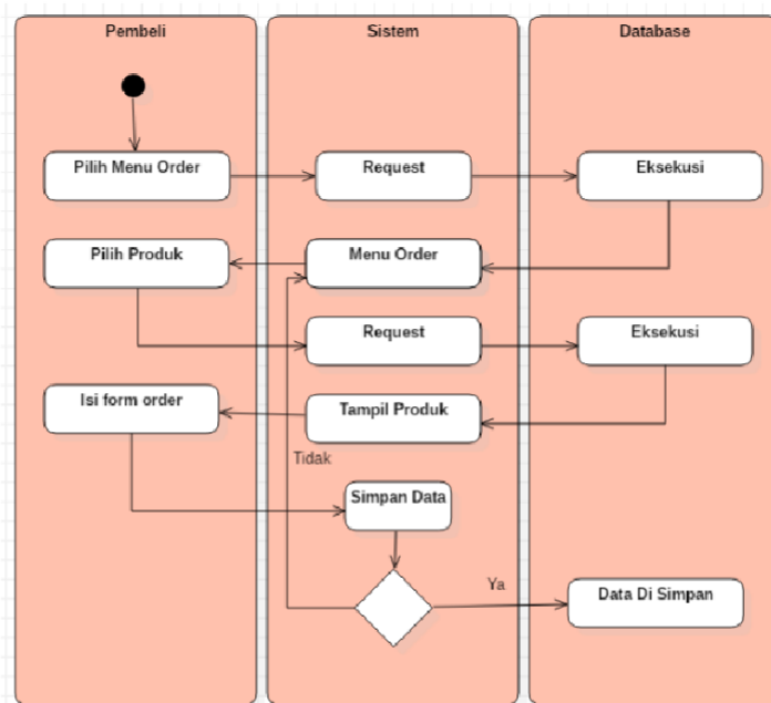
Gambar 3. Activity Diagram.
