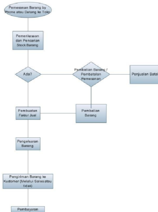
Gambar 1. Flowchart
