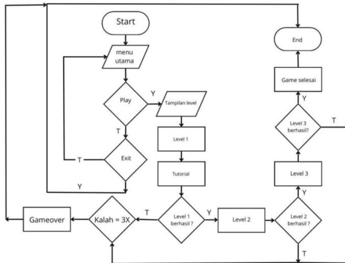
Gambar 2. Flowchart Game
