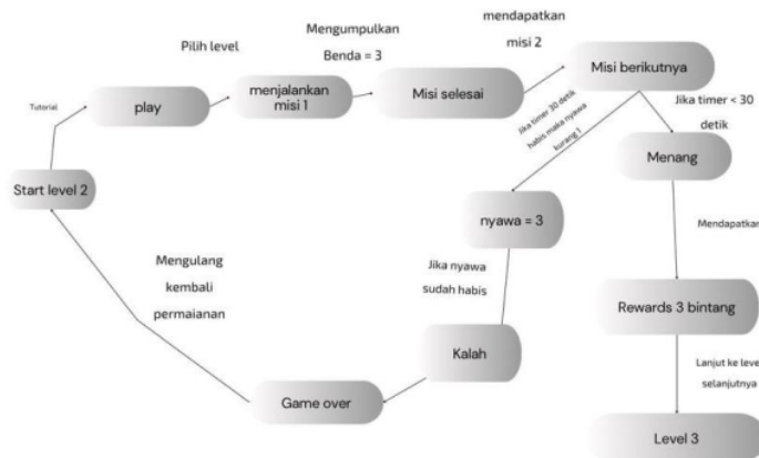
Gambar 5. Diagram Finite State Machine Level 2
