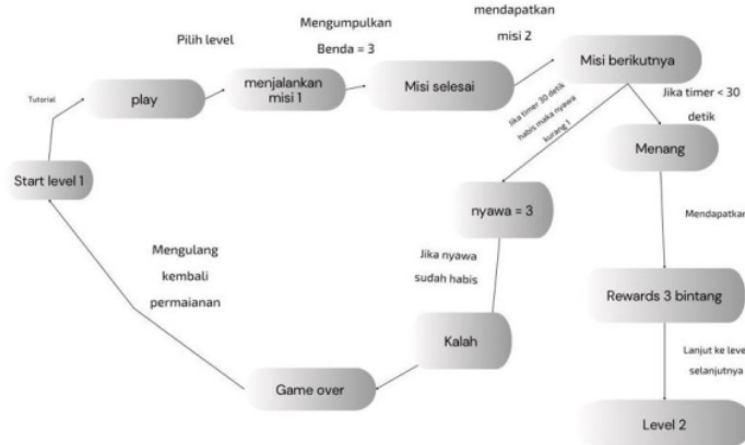
Gambar 4. Diagram Finite State Machine Level 1
