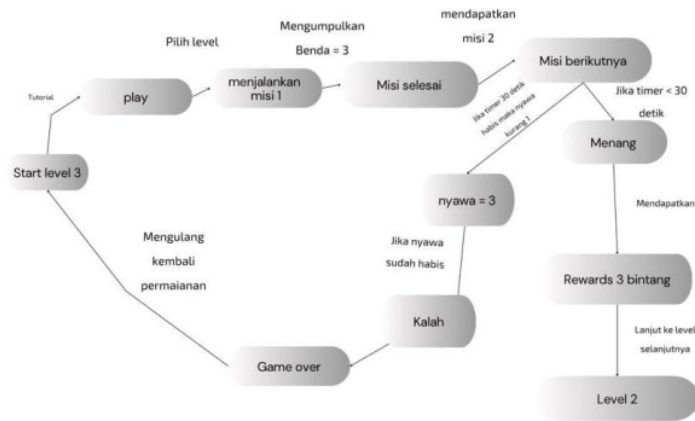
Gambar 6. Diagram Finite State Machine Level 3
