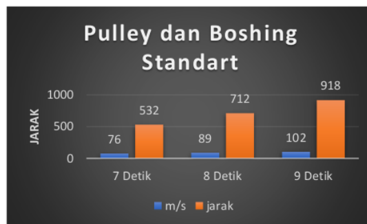
Gambar 1 Grafik Top Speed dan Jarak Pulley, Boshing Standart
