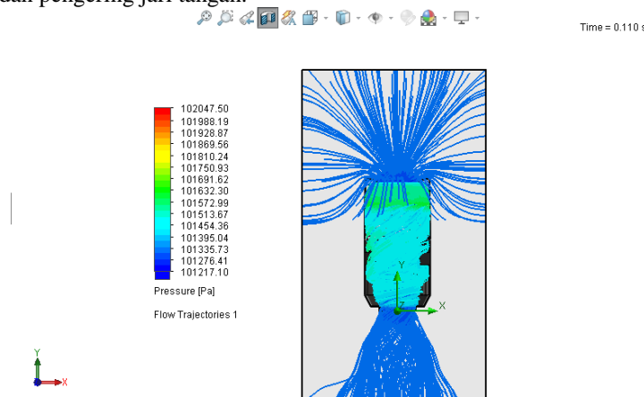
Gambar 4. Simulasi Pressure
