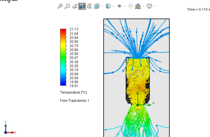
Gambar 6. Simulasi Temperature
