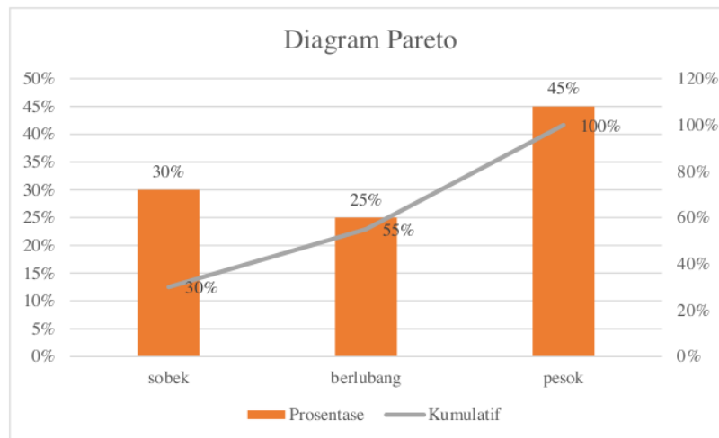
Gambar 3. Diagram Pareto
