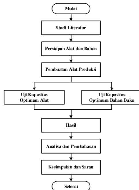
Gambar 1. Flowchart Penelitian
